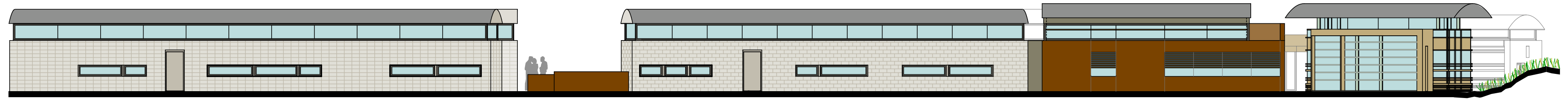
NORTH ELEVATION
